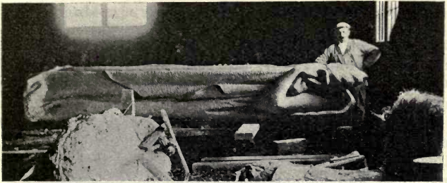
FIG. 47—STATUE FINISHED EXCEPT FOR HEAD AND PROJECTING PORTIONS OF FEET, SEPARATELY CAST
